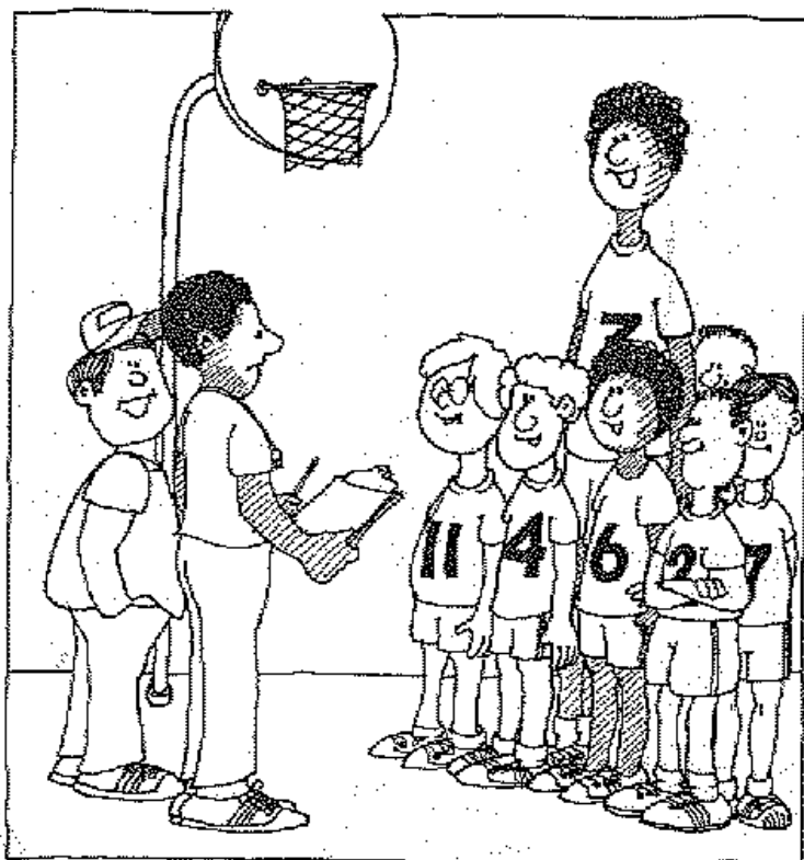
1. Measuring center or average
