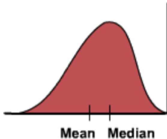
Left (or Negative) skewed
